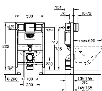
Rapid SL 0.82m Installation Height
