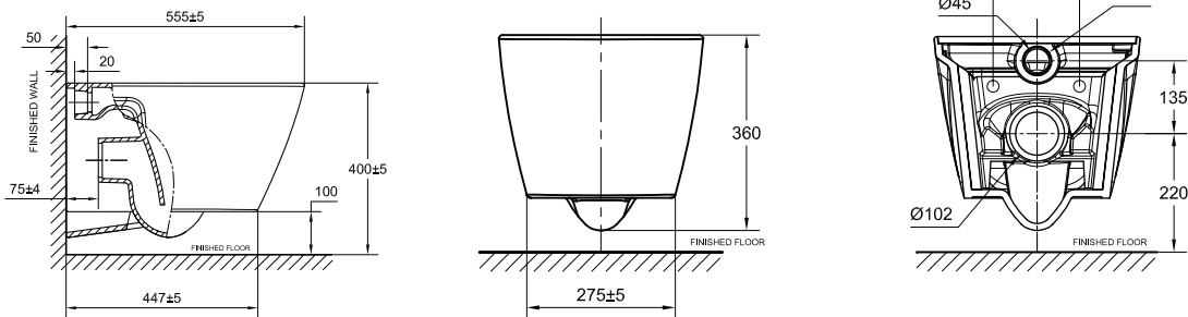
Acacia SupaSleek Wall Hung WC
