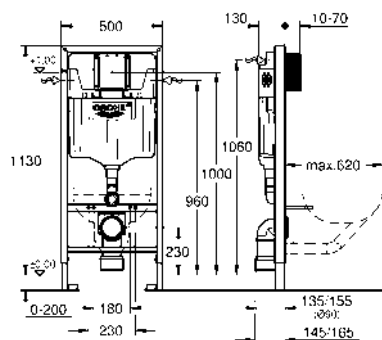
Rapid SL 1.13m Installation Height
