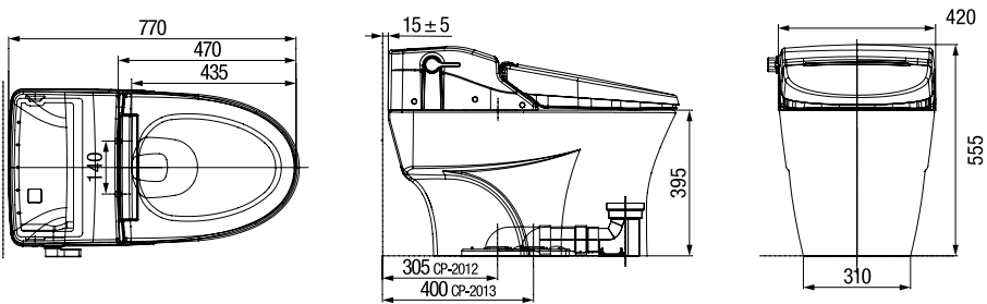
AEROZEN Shower Toilet
