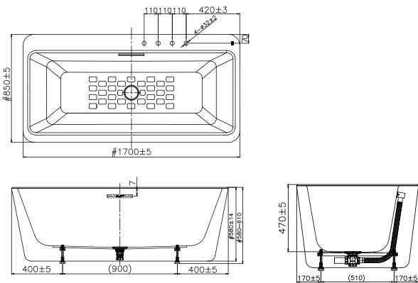
Acacia Evolution 1.7M Acrylic Seamless Freestanding Tub (with Faucet Installation Holes)
