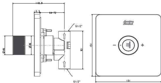
EasySET for Body Shower FFAS0927-709500BC0
