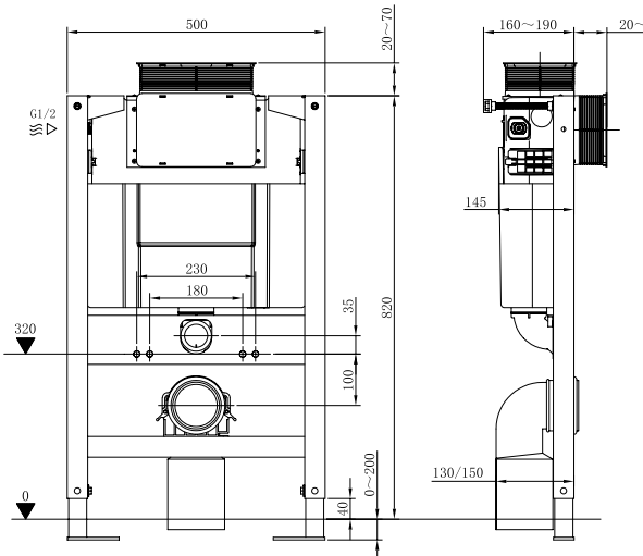
Repelo Concealed Cistern with Frame Height 820mm
