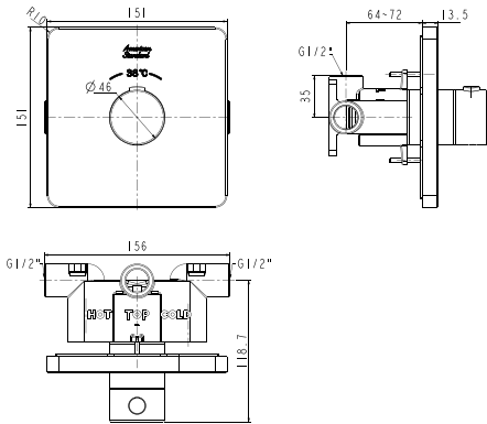
EasySET Concealed Thermostatic Mixer with Trim FFAS0930-000500BC0
