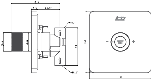
EasySET for Head Shower FFAS0926-709500BC0
